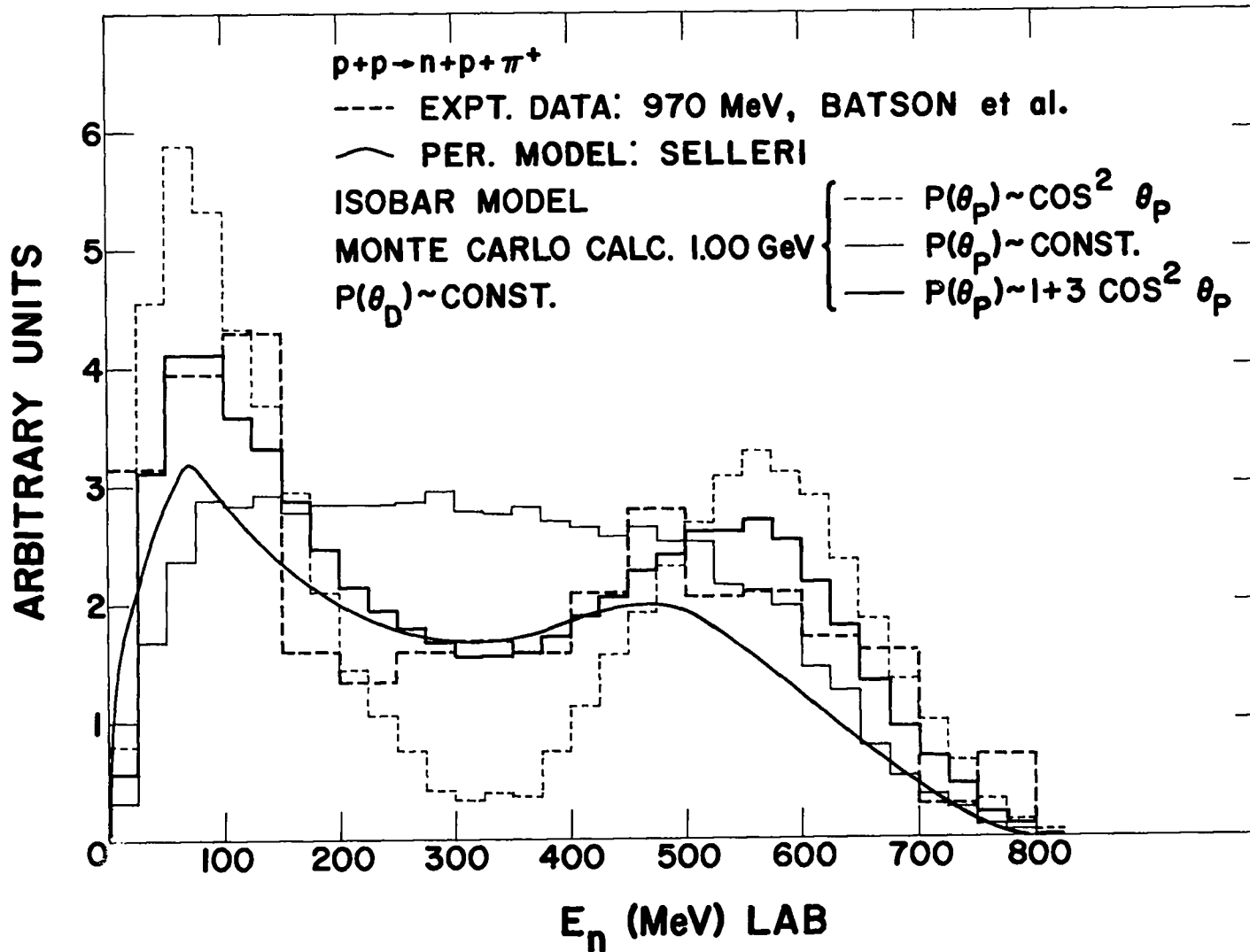
Figure 2. Comparison of isobaric nucleon model calculations with the neutron energy spectra from the reaction p+p \rightarrow n+p+\pi^+ at 970 MeV. Data (heavy dashed line) are from Batson et al. 7 Peripheral model calculation of Selleri 7 is also shown.
