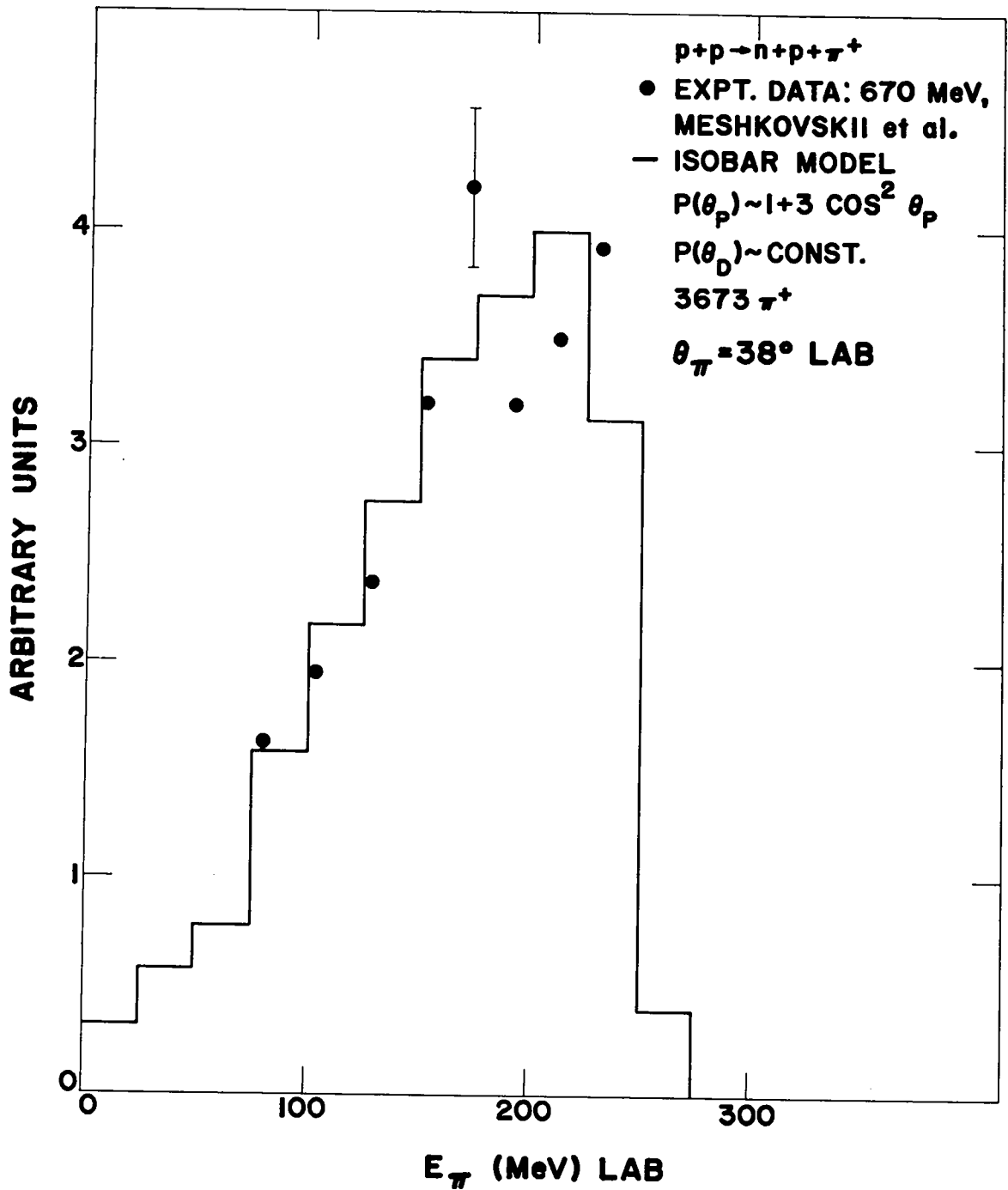
Figure 4. Comparison of isobaric nucleon model calculation with observed pion energy spectra of Meshkovskii et al. 17 from p+p \rightarrow n+p+\pi^+ at 670 MeV and \theta_\pi = 38^\circ Lab.
