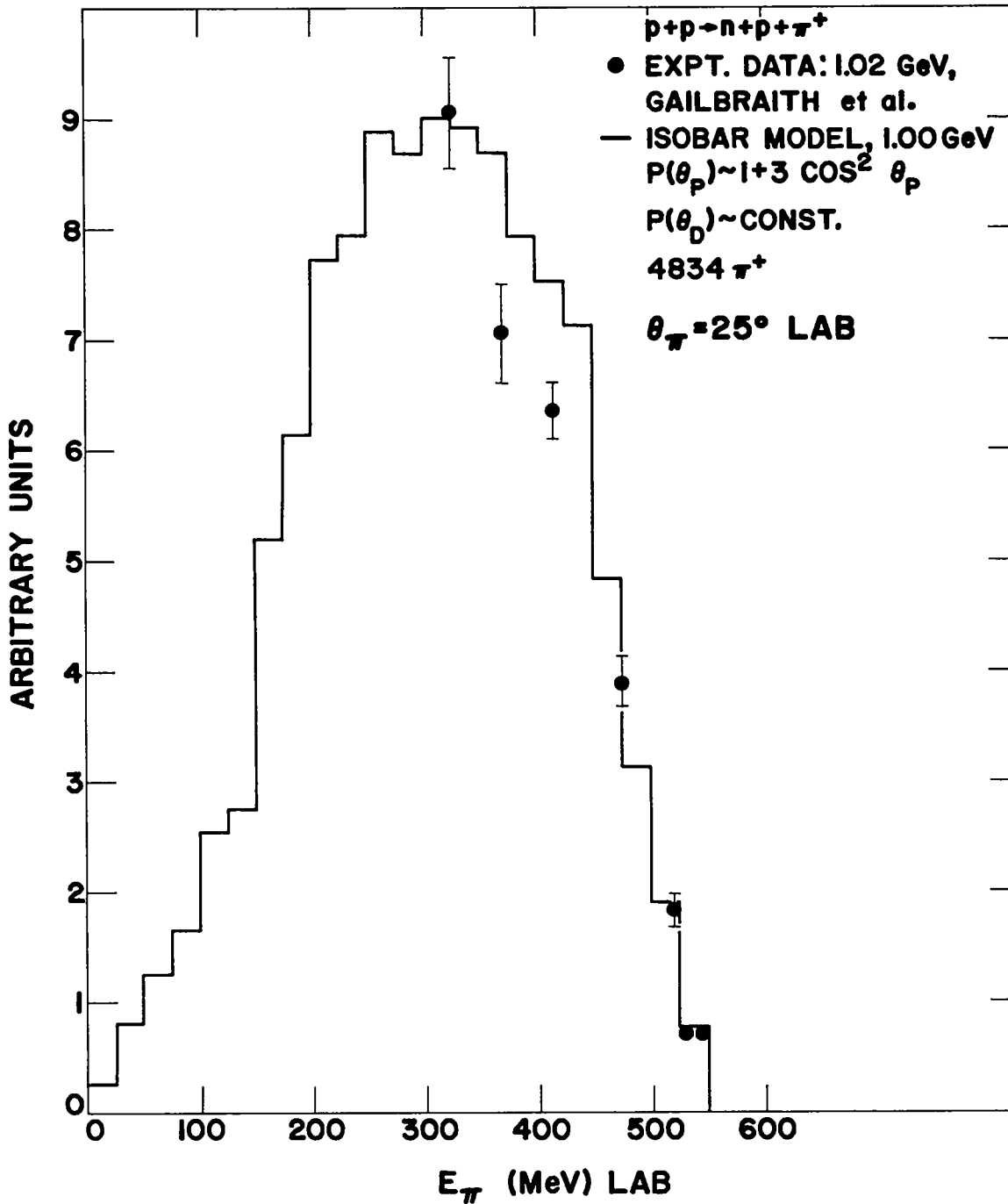
Figure 7. Comparison of isobaric nucleon model calculation with observed pion energy spectra of Gailbraith et al. 10 from p+p \rightarrow n+p+\pi^+ at 1.02 GeV and \theta_\pi = 25^\circ \text{ Lab} .
