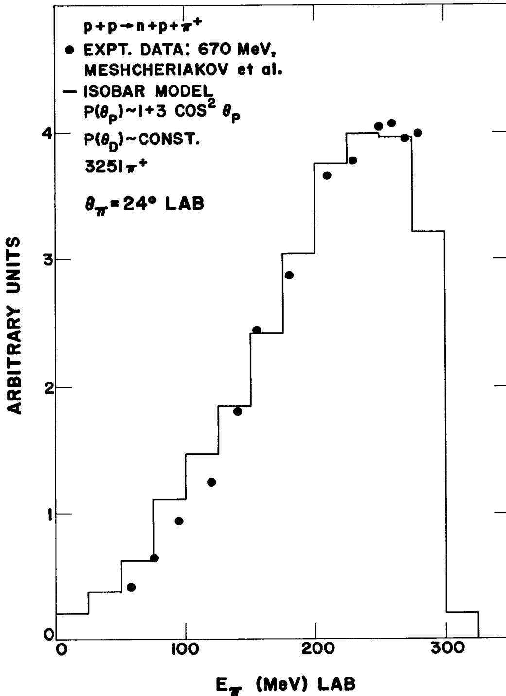
Figure 3. Comparison of isobaric nucleon model calculation with observed pion energy spectra of Meshcheriakov et al. 16 from p+p \rightarrow n+p+\pi^+ at 657 MeV (not 670 MeV as shown above on Fig.) and \theta_\pi = 24^\circ \text{ Lab} .
