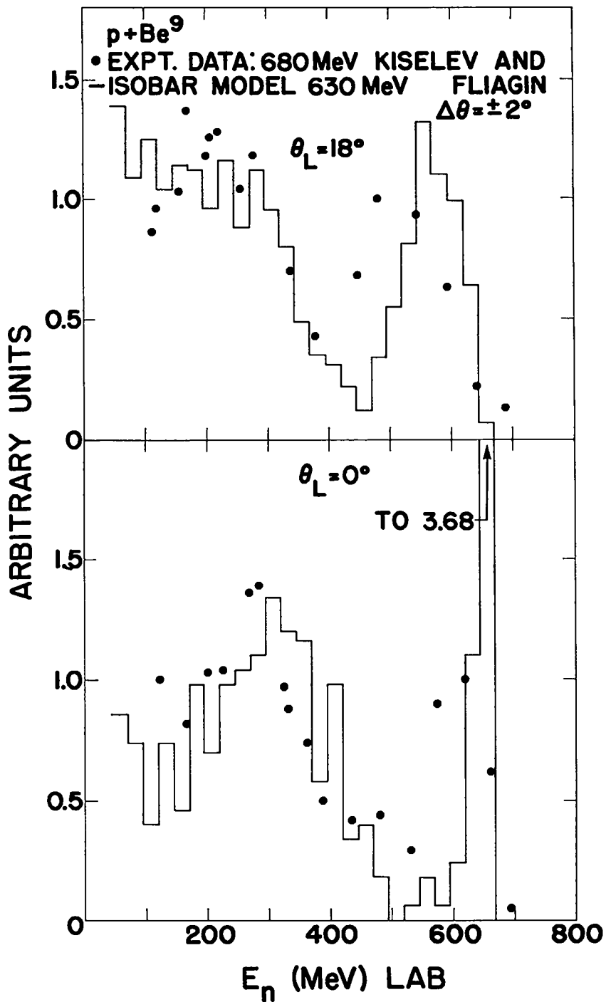
Figure 9. Comparison of Maniac II intranuclear cascade calculation with observed neutron energy spectra of Kiselev and Fliagin 14 from p+Be^9 at 680 MeV and \theta_n = 0^\circ and 18^\circ Lab.
