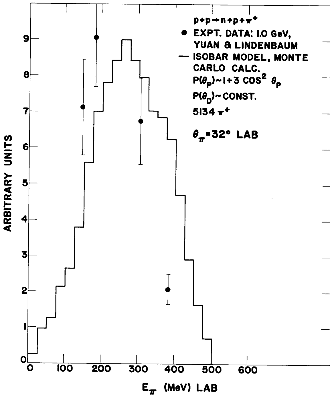
Figure 8. Comparison of isobaric nucleon model calculation with observed energy spectra of Yuan and Lindenbaum, from p+p \rightarrow n+p+\pi^+ at 1.0 GeV and \theta_\pi = 32^\circ \text{ Lab} .
