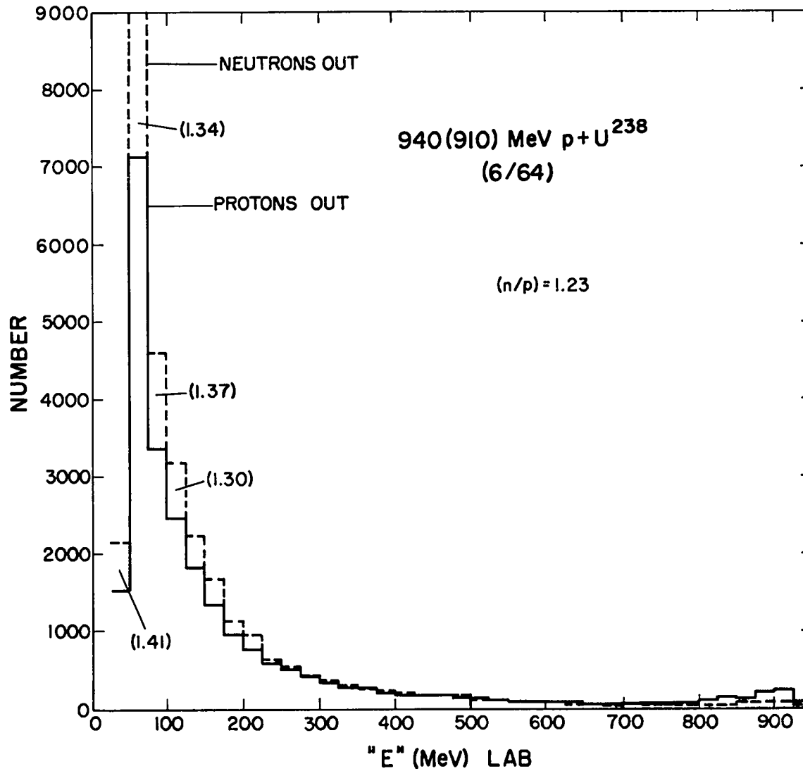
Figure 13. Maniac II calculation of neutron and proton energy spectra from 910 MeV protons incident on U 238 . "E" is the energy of the particles just before escaping from the nuclear boundary; shift distribution by -30 MeV to obtain outgoing energy spectra.
