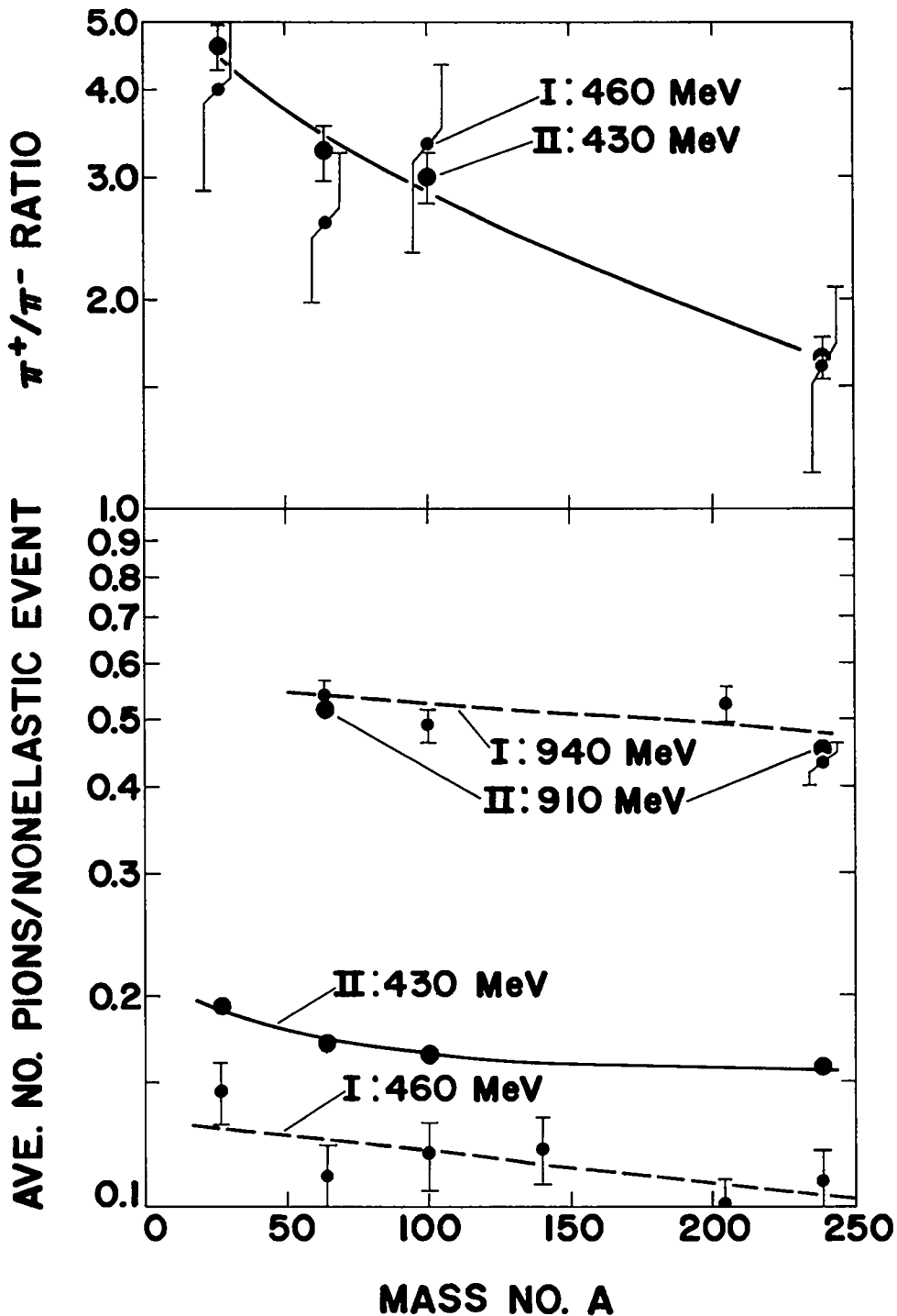
Figure 15. Comparison of Maniac I and Maniac II calculations: a) average number of pions per nonelastic event and b) \pi^+/\pi^- ratio, both as functions of target mass number A, and for incident proton energies of about 445 and 925 MeV.
