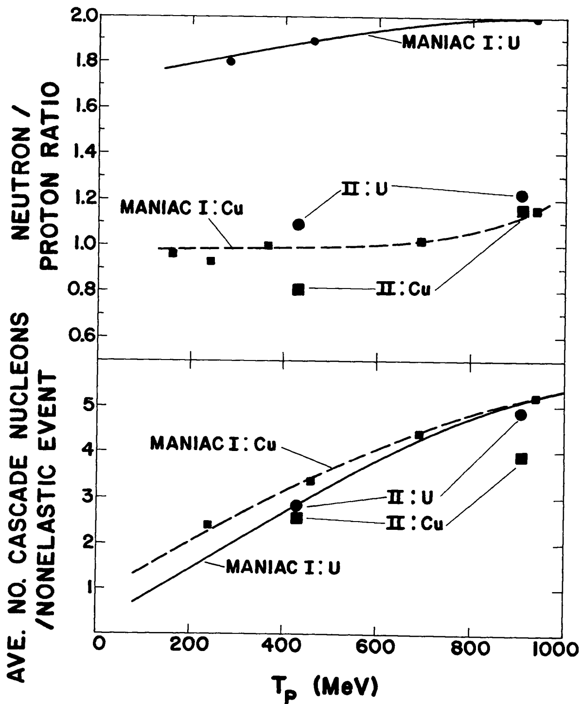
Figure 11. Comparison of Maniac I 2 and Maniac II calculations: a) average number of cascade nucleons per nonelastic event and b) the neutron/proton ratio, both as functions of incident proton energy T_p and for \text{Cu}^{64} and \text{U}^{238} targets.
