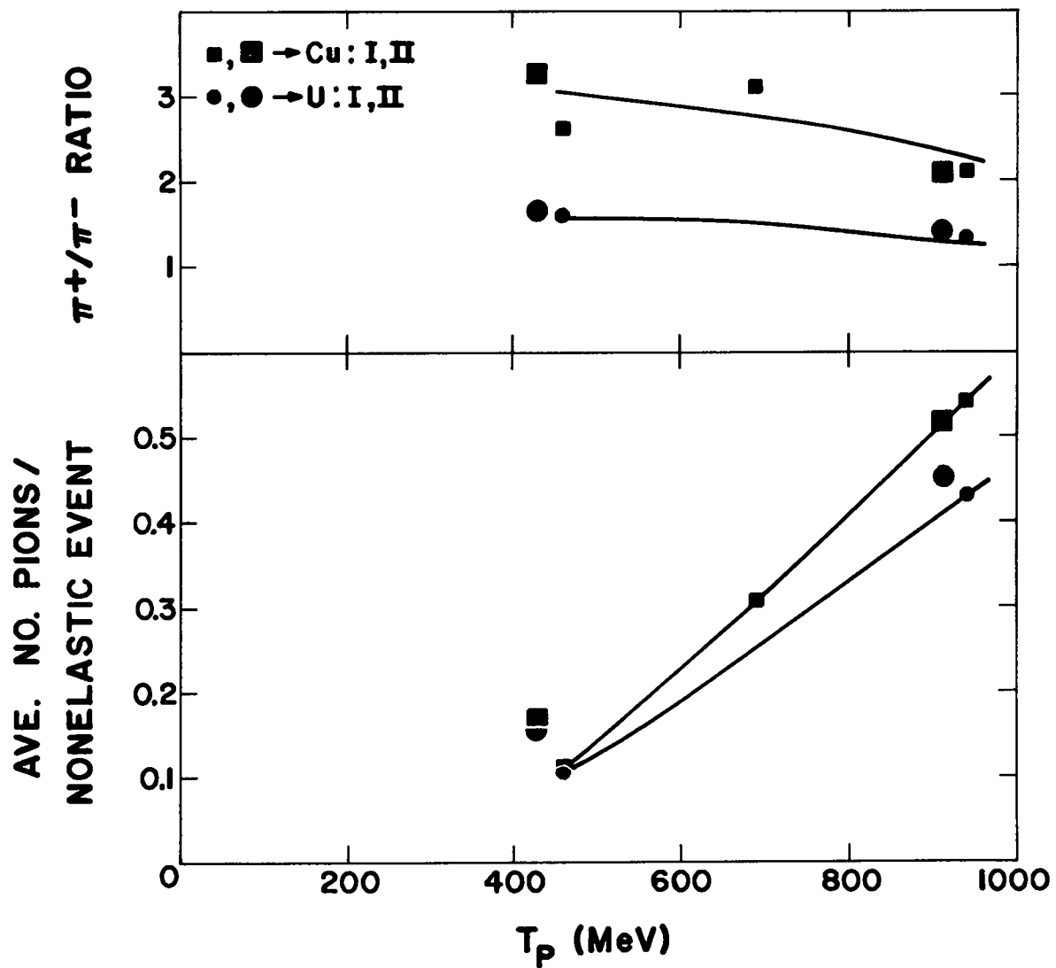
Figure 14. Comparison of Maniac I and Maniac II calculations: a) average number of pions per nonelastic event and b) \pi^+/\pi^- ratio, both as functions of incident proton energy T_p and for \text{Cu}^{64} and \text{U}^{238} targets.
