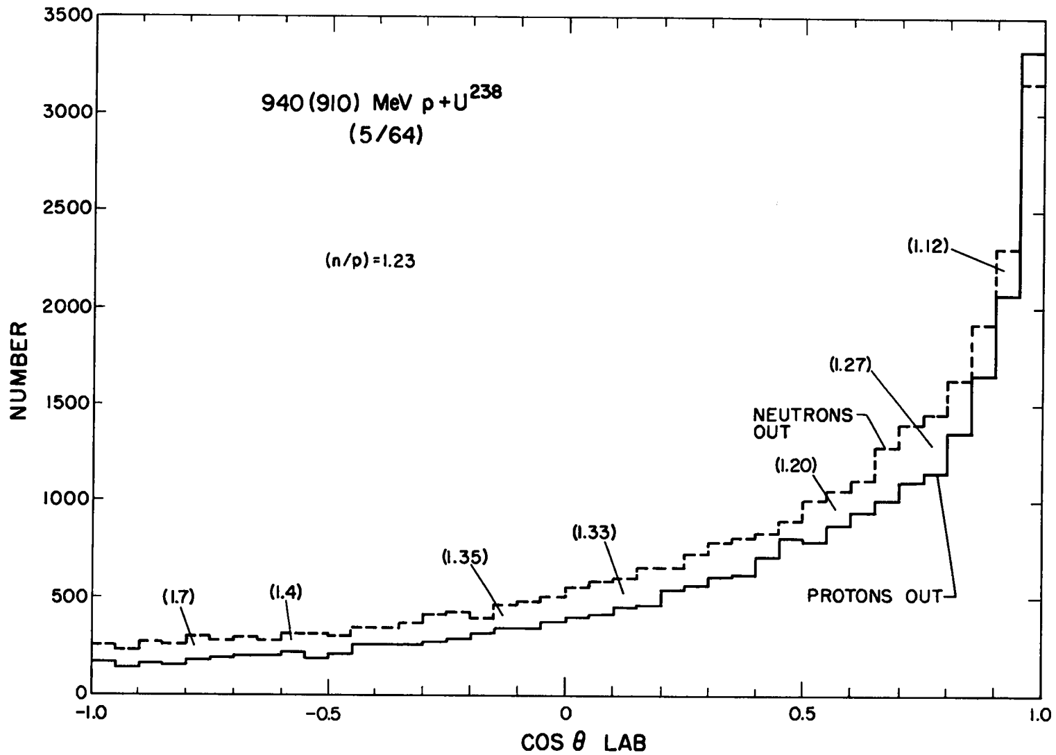
Figure 12. Maniac II calculation of neutron and proton angular distributions from 910 MeV protons incident on U 238 (assumes a square-well potential of 30 MeV; protons just inside nuclear boundary have 940 MeV).
