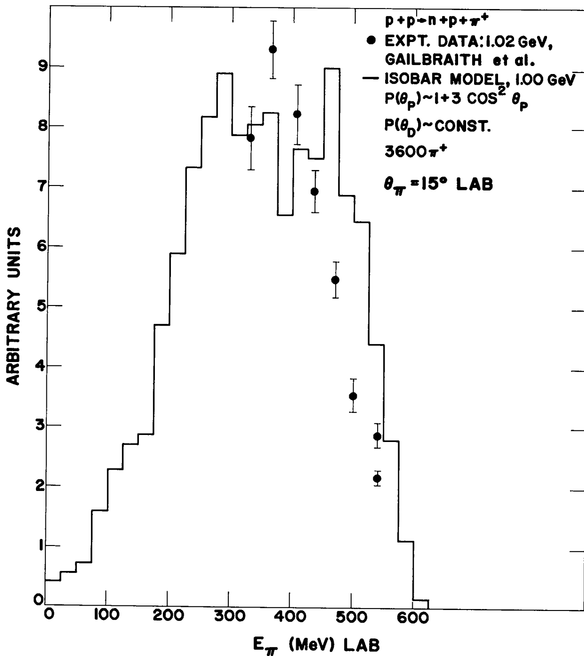
Figure 6. Comparison of isobaric nucleon model calculation with observed energy spectra of Gailbraith et al. 10 from p+p \rightarrow n+p+\pi^+ at 1.02 GeV and \theta_\pi = 15^\circ \text{ Lab.}
