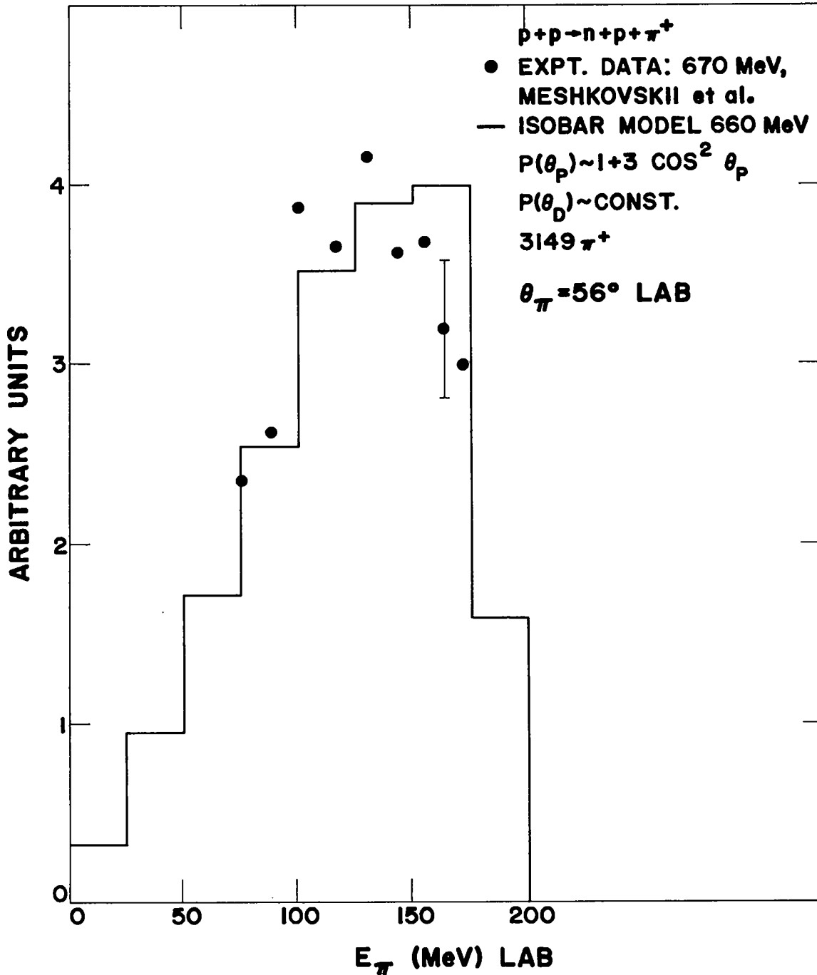
Figure 5. Comparison of isobaric nucleon model calculation with observed pion energy spectra of Meshkovskii et al. 17 from p+p \rightarrow n+p+\pi^+ at 670 MeV and \theta_\pi = 56^\circ Lab.
